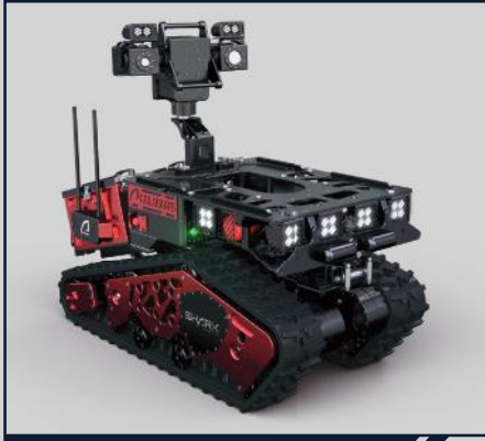
VIDEO TURRET 180°
